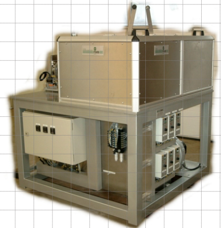
Feeder for providing 3 kinds of sockets
