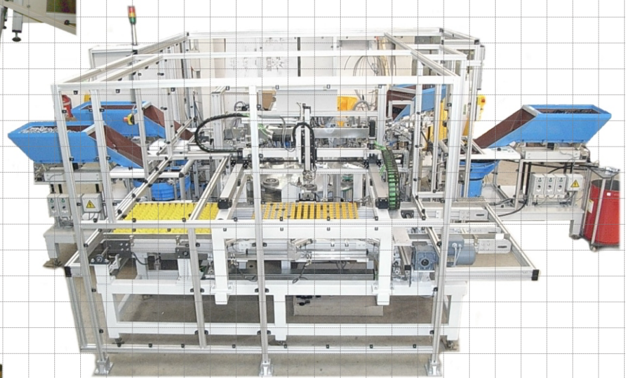
Assembly machine for sealing cap
