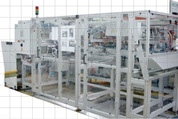
Total system with storage and ejection of finished parts
