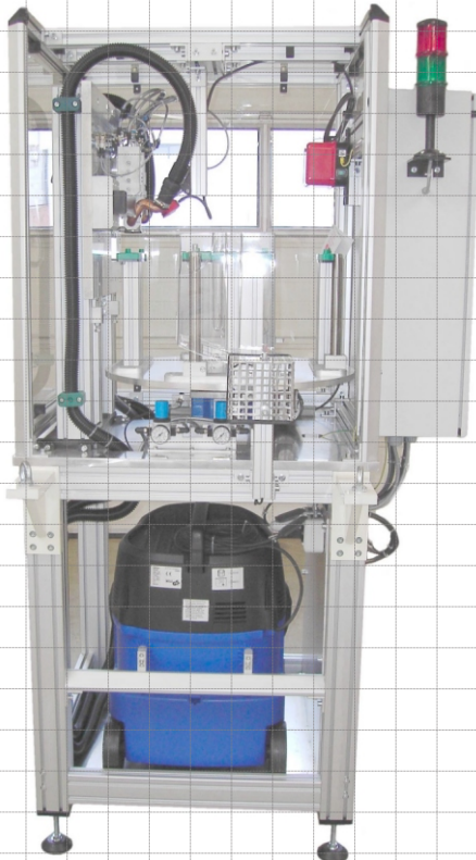
Rotary indexing machine for plastic parts
