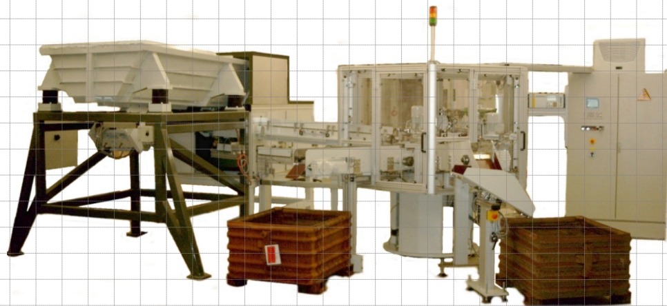
Rotary indexing machine for testing various studs.
