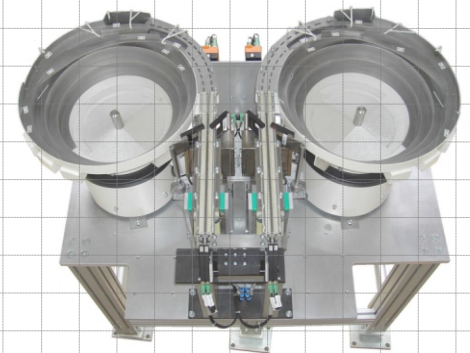
2-fold supply & provision for rubber parts
